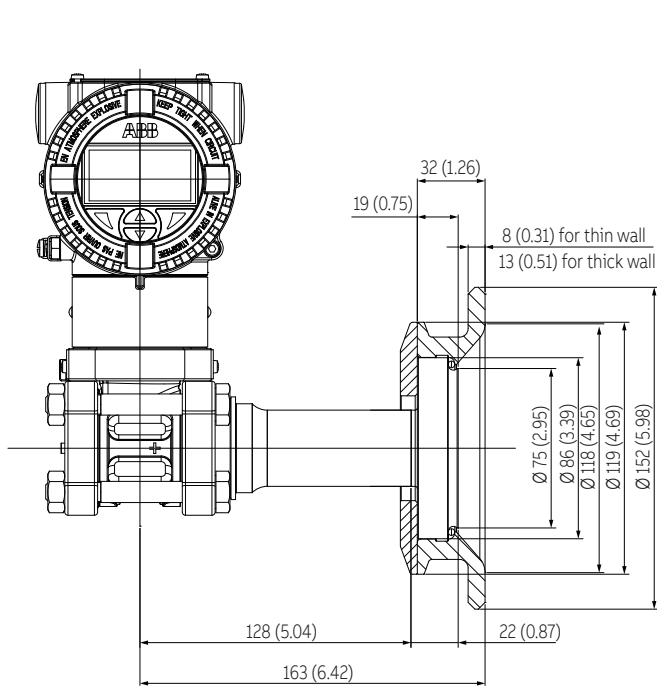
Figure 28 266DRH with barrel housing and direct mount seal S26SS Sanitary flush (For dimensions of S26 seals refer to the S26 datasheet)
