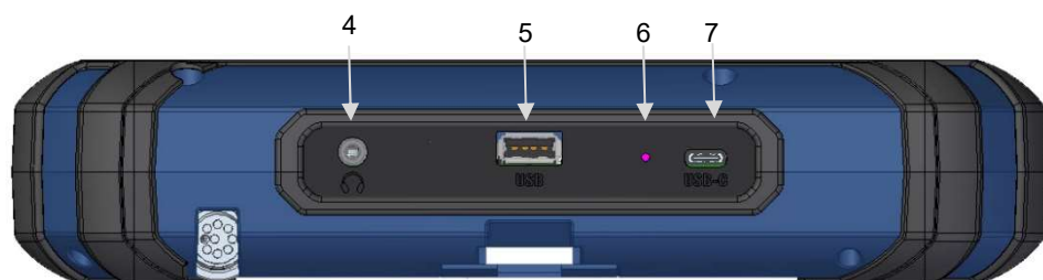
Fig. 8: Bottom side of the monitor with terminal strip
